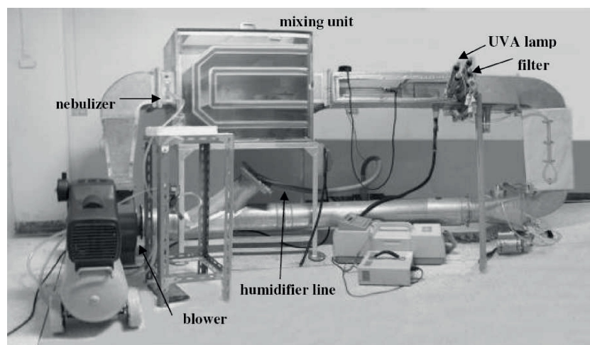
Figure 1. The closed-loop chamber
