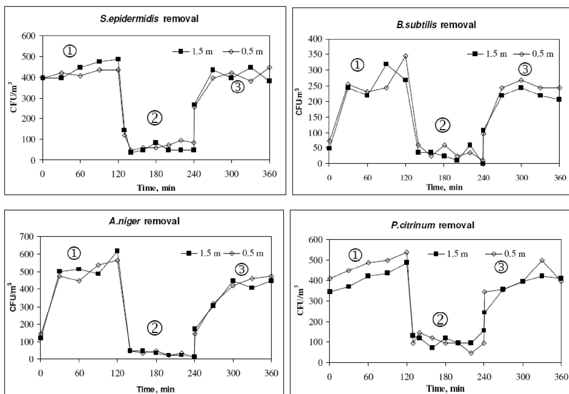
Figure 4. Disinfection efficiency of PCO air purifier in the 8-m 3 chamber at two different heights: ① = before turning on the air purifier, ② = while turned on, and ③ = after turning off the air purifier
