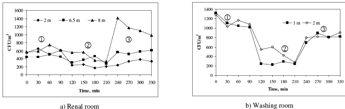
Figure 5. Disinfection efficiency of PCO air purifier at different distances from the air purifier in a renal room and a washing room in a hospital: ① = background concentration, ② = during operation of the air purifier, and ③ = after turning off
