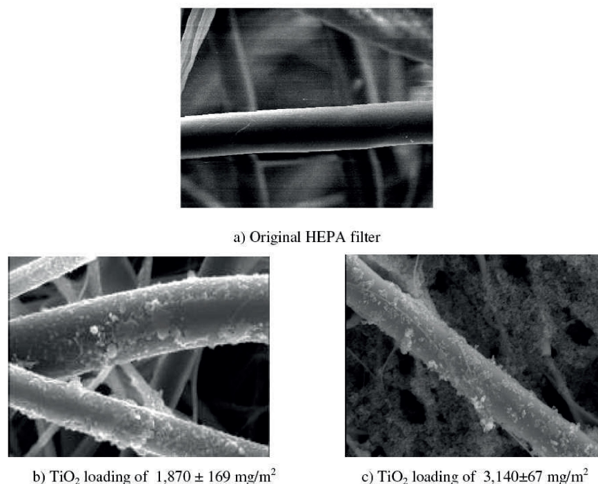
Figure 2. Morphology of fibers under various conditions (5,000× magnifications for all micrographs)
