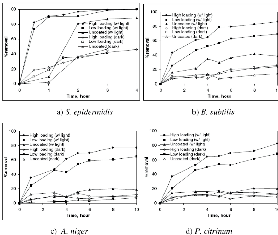
Figure 3. Disinfection efficiency of photocatalytic HEPA filters in the closed-loop chamber
